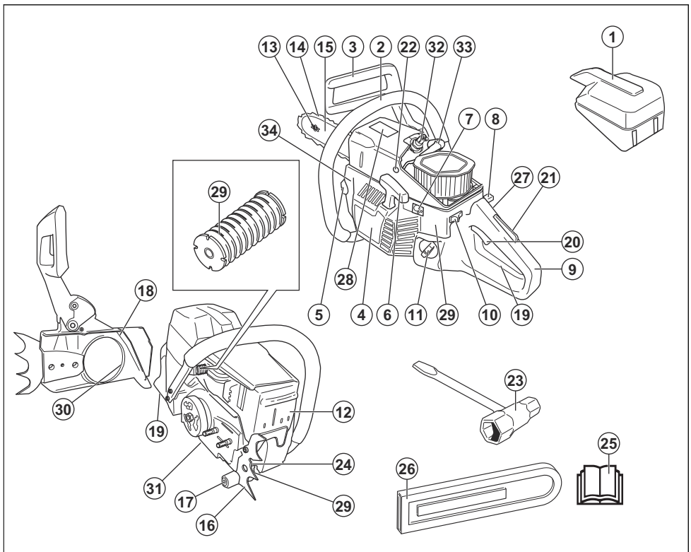
1. Air filter cover
